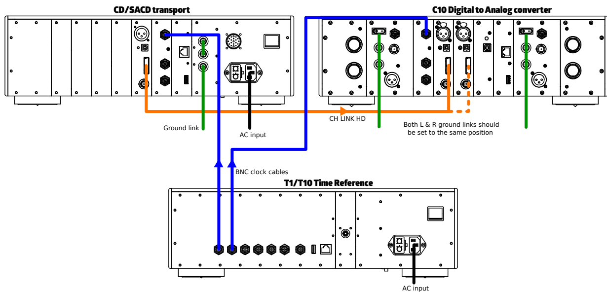
CD/SACD transport - C10 - T1/T10 connection when CLOCK_SYNC equipped
